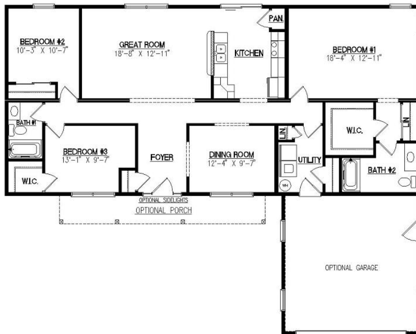
First Floor (w/ Crawl Space)
