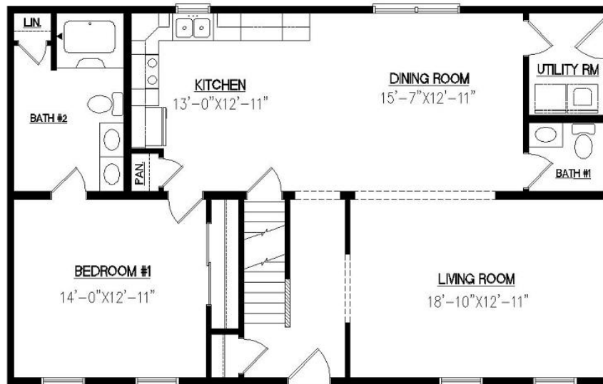
First Floor (w/ Basement)
