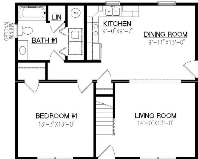
First Floor (w/ Crawl Space)
