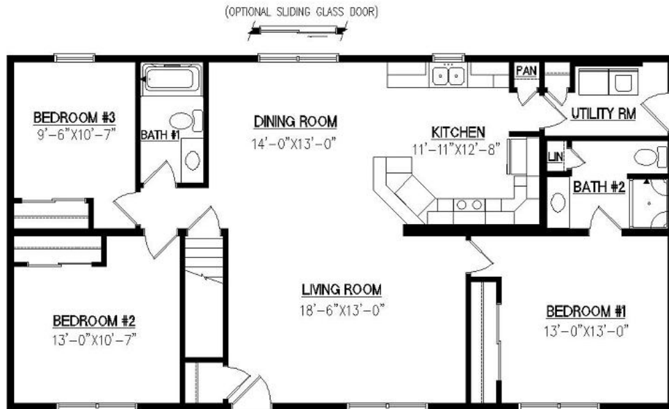
First Floor (w/ Basement)
