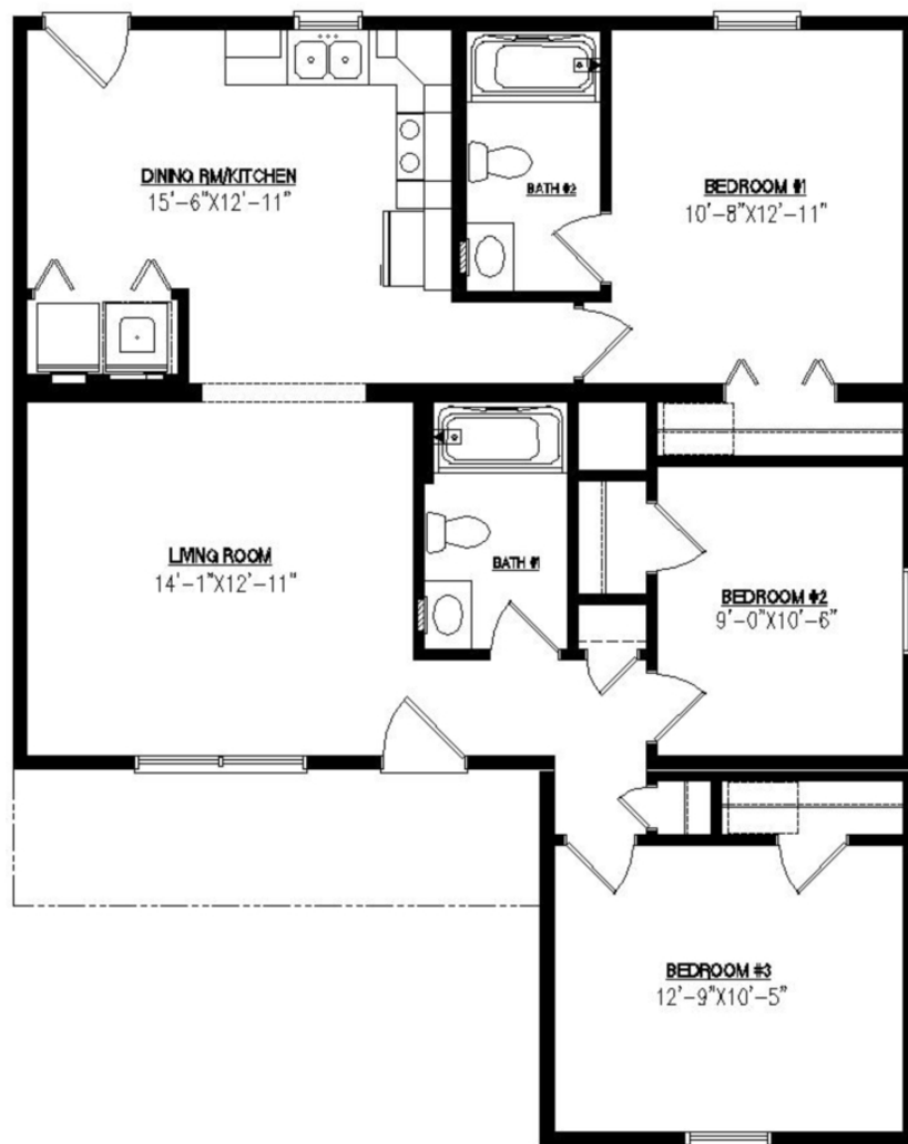
First Floor (w/ Crawl Space)
